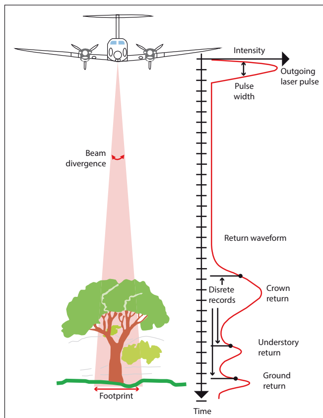
Figure 7.3. Visualization of Lidar Technology
