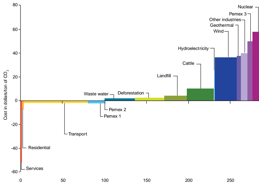
Figure VII.26 MEXICO: MARGINAL COST CURVE OF MITIGATION, 2020 (Millions of tons of CO 2 per year)
