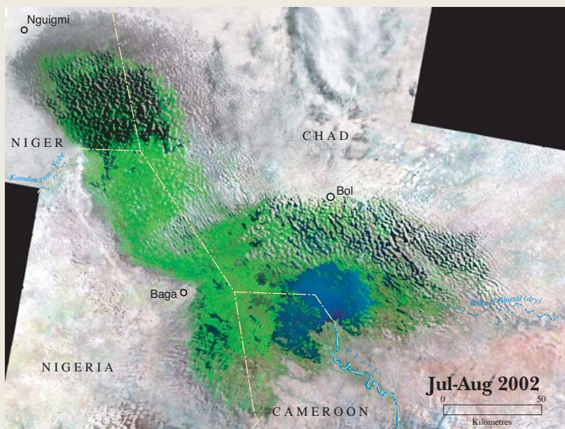
Figure 3.2: Landsat images of Lake Chad: Jul-Aug 2002, Nov-Dec 2002, Feb 2003 and May 2003
