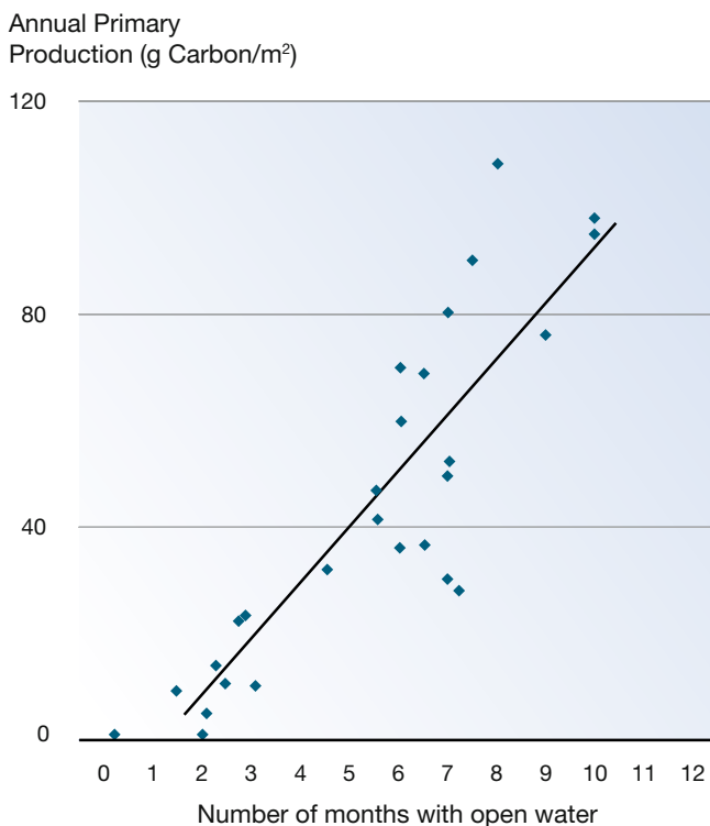
Figure 16.1: The relationship between annual primary production and the ice-free period based on measurements from several sites in the Arctic [9].
