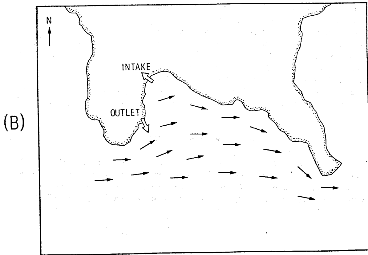
Figure 3. Generalized patterns of tidal currents in Nanwan Bay for (A) flood tide and (B) ebb tide
