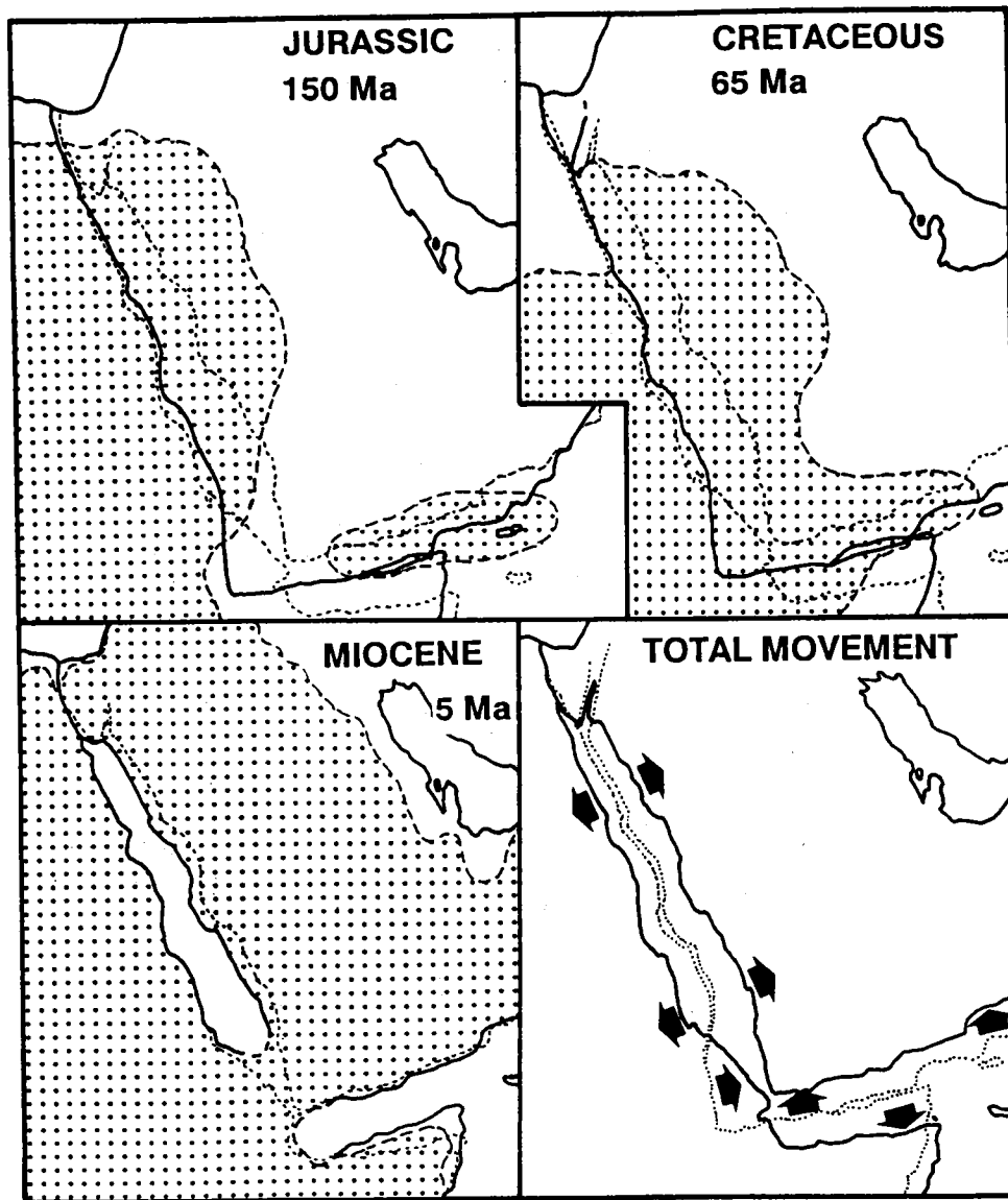
Figure 4: Palaeogeography of Red Sea in Jurassic, Cretaceous and Miocene Periods
