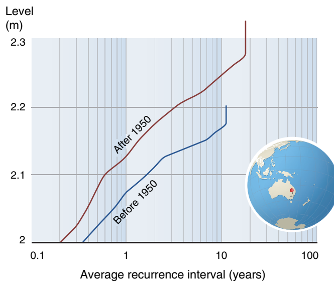
Figure 6C.7: Average Recurrence Interval for sea-level events of a given height at Sydney, Australia. For the second half of the 20th century (red line), the average recurrence interval for a sea-level height of a given value is less than half the value for the first half of the 20th century (blue line).
