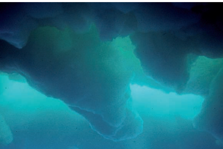
Figure 5.15a: Underside of multi-year sea ice. Photo: Haakon Hop, Norwegian Polar Institute
