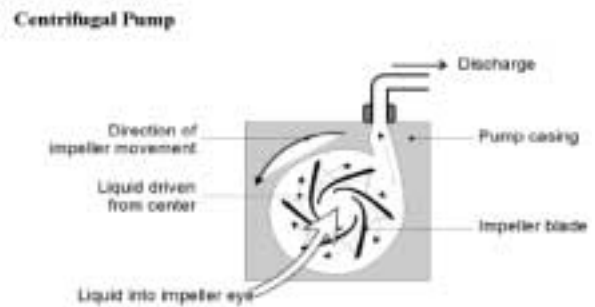
Figure 15: pompe centrifuge
