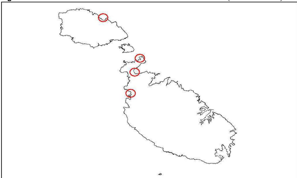
Figure 3 Location of the extant sand dunes in the Maltese Islands (Source: MEPA)
