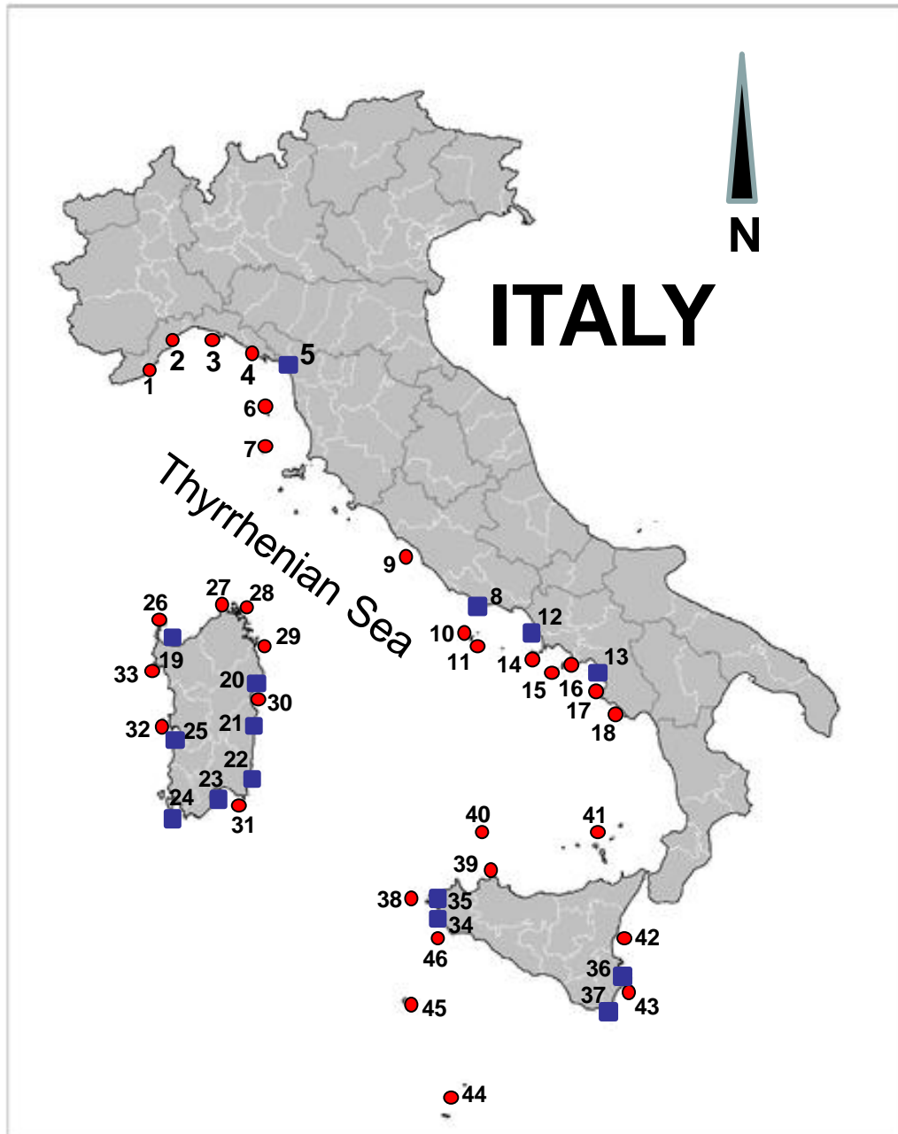
Figure 1 List of marine and coastal sites considered to be especially at risk (or endangered) in the short term by the effects of climate change in Italy (Adriatic excluded). Squares refer to Areas at risk from rises in sea level and circles refer to areas at risk of impact on biodiversity.
