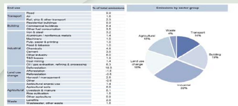
Figure 7.1: Sector contributions to global GHG emissions
