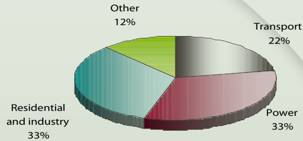
Chart 1: Main sources of CO 2 emissions
