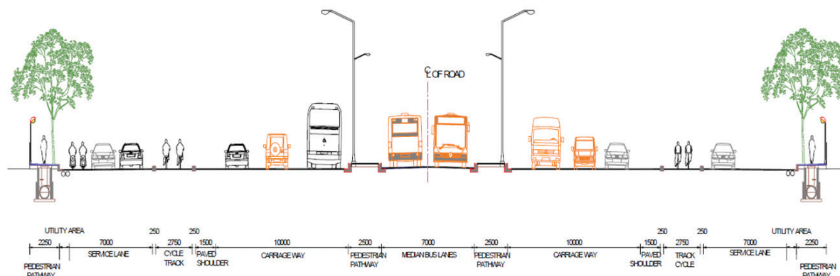
Figure 4.3 Road section at 60 m ROW
