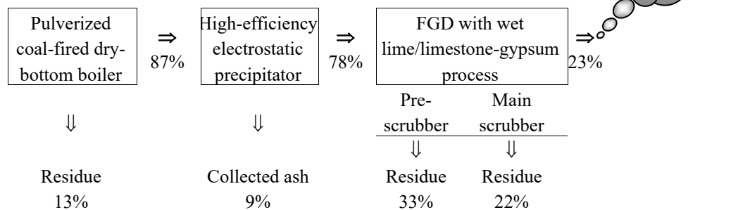
Figure 5-1 Reducing mercury emissions with wet FGD systems; mercury flows and outputs in % of mercury input to boiler based on Pacyna and Pacyna (2000) (figure from UNEP, 2002)
