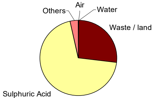
Figure 5-4 The mercury output distribution from a Canadian zinc/copper smelter with low mercury inputs and no mercury specific emission abatement (UNEP, 2011).
