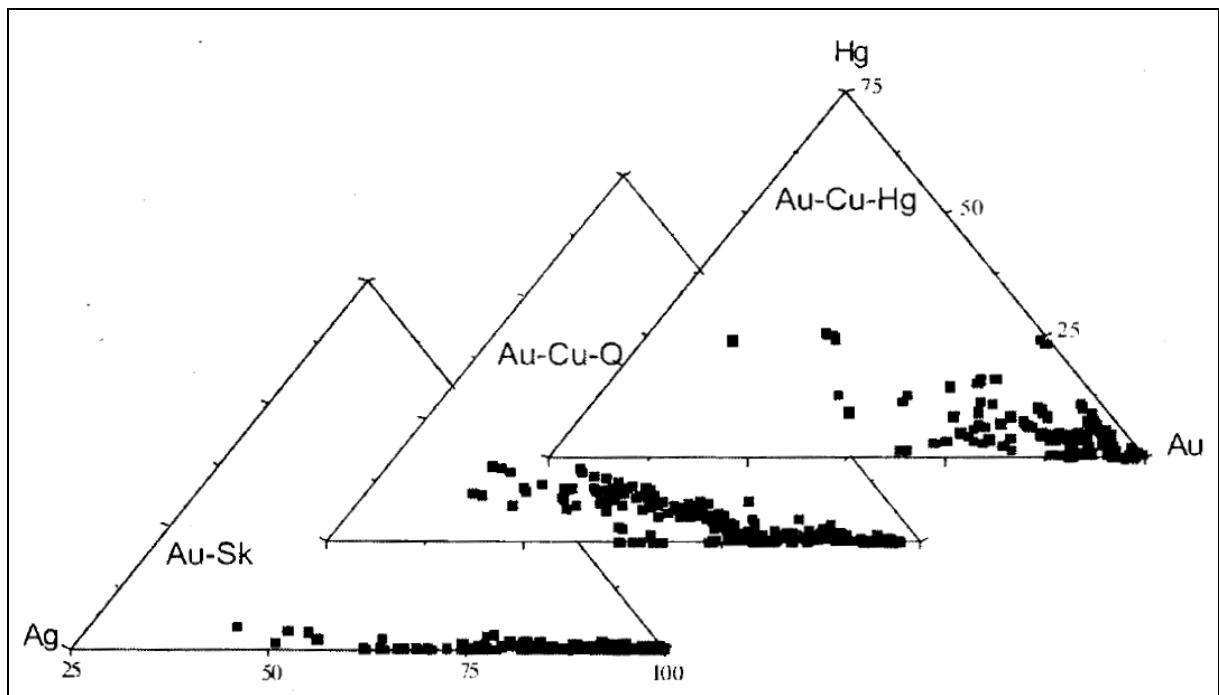
Figure 5-9 Mercury, gold and silver concentrations in natural gold grains of gold-skarn, gold-copper-quartz and gold-copper-mercury mineral types from (Borisenko et al, 2004).
