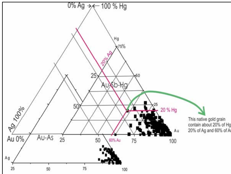
Figure 5-8 Mercury, gold and silver concentrations in natural gold grains of gold-antimony-mercury and gold-silver mineral types (from Borisenko et al (2006) with help for reading the figure from Naumov, 2019).
