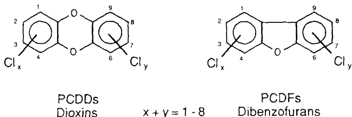
Fig. 1. Structural formulae of PCDDs and PCDFs.
