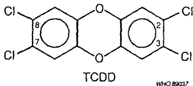
Fig. 2. Structural formula of TCDD.
