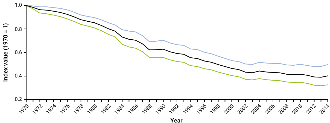
Figure SPM.2. Global Living Planet Index
