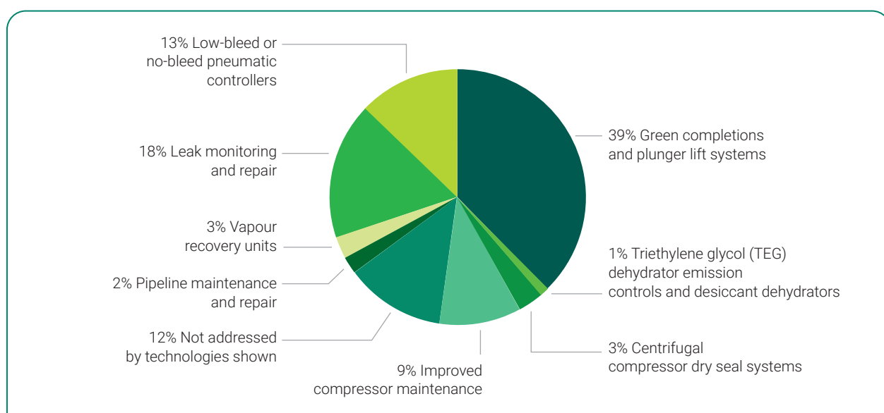
FIGURE 3.5: TECHNOLOGIES WITH THE GREATEST POTENTIAL TO REDUCE METHANE EMISSIONS IN THE OIL AND GAS INDUSTRY
