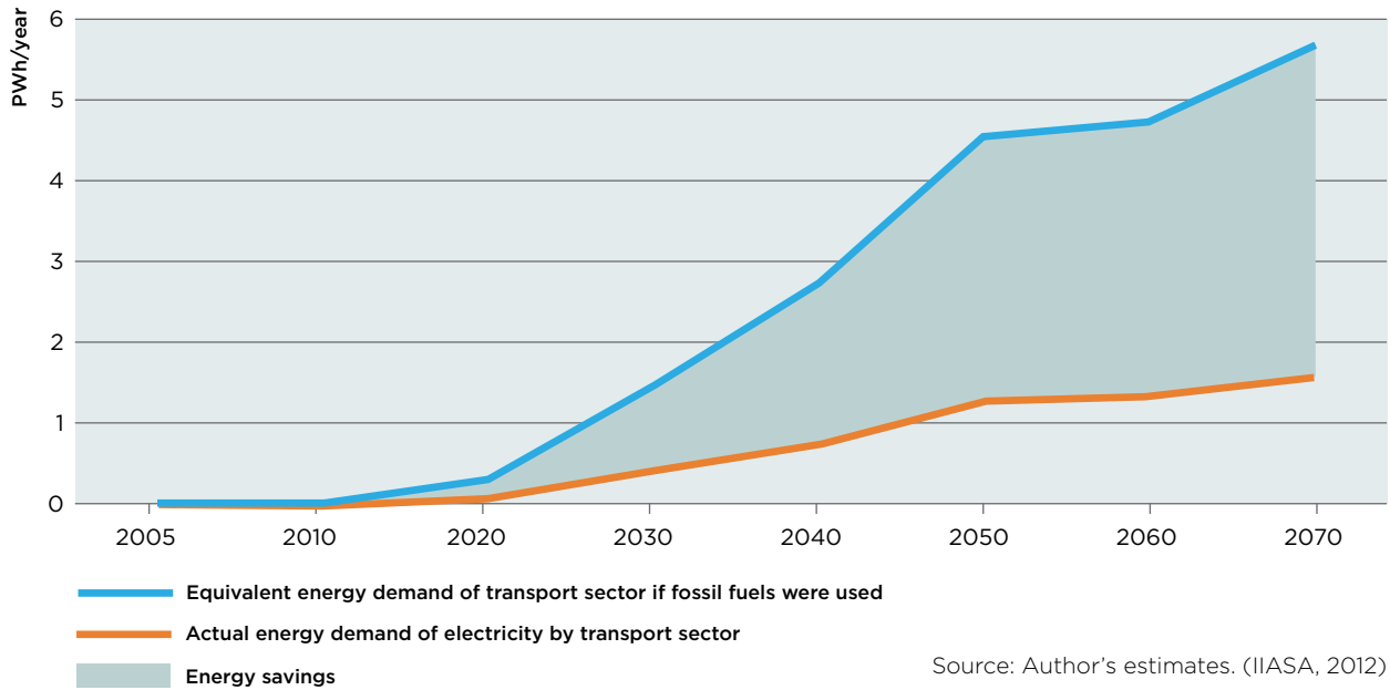
Figure 3.15 - Energy savings from full transport electrification.
