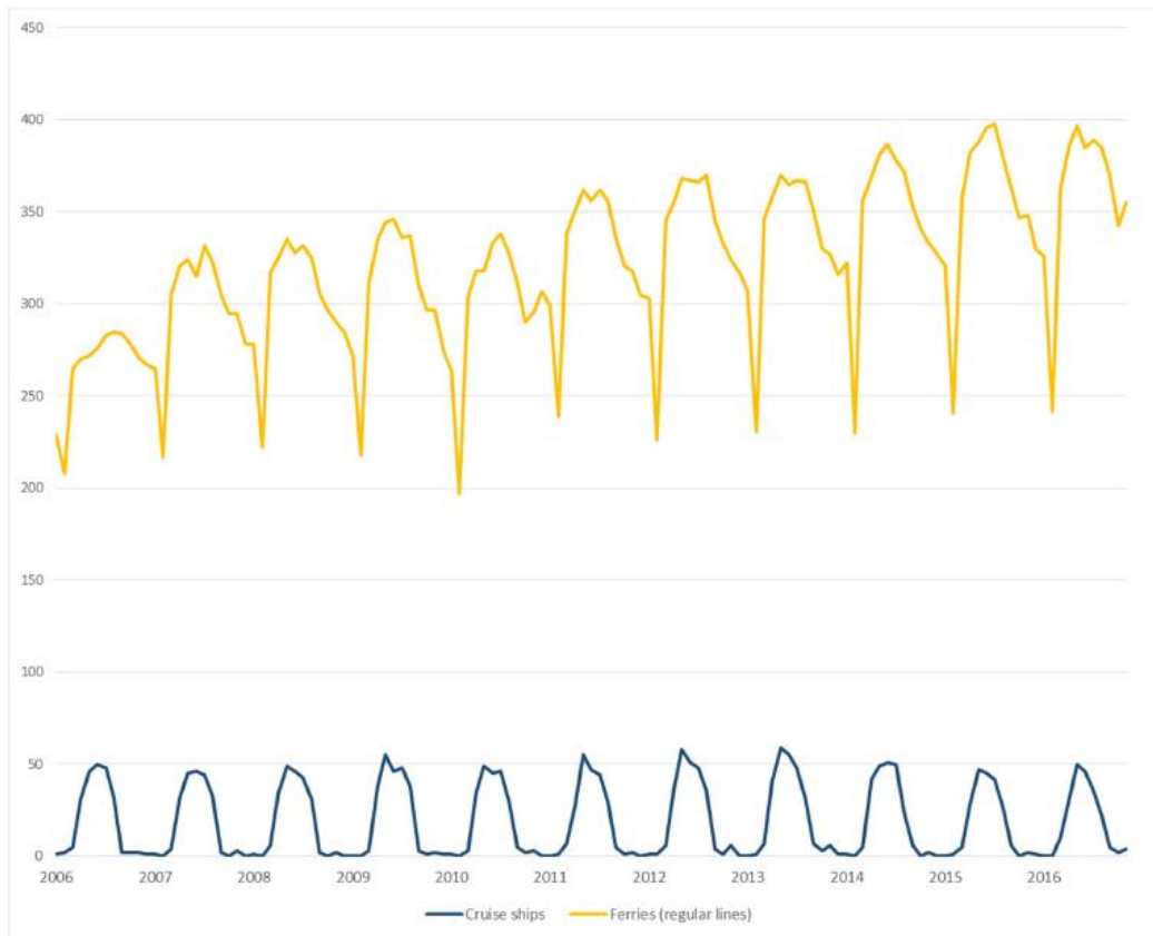
Figure 3: Number of cruise ships and ferries 28 operating in the Baltic Sea (monthly values) based on the HELCOM AIS data (source: HELCOM Baltic Marine Environment Protection Commission)
