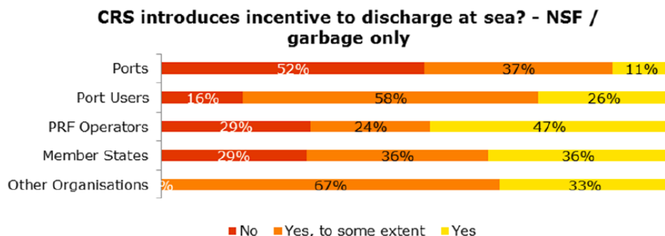
Figure 12: Incentives to discharge waste at sea in NSF for garbage only (source: Panteia/PwC)
