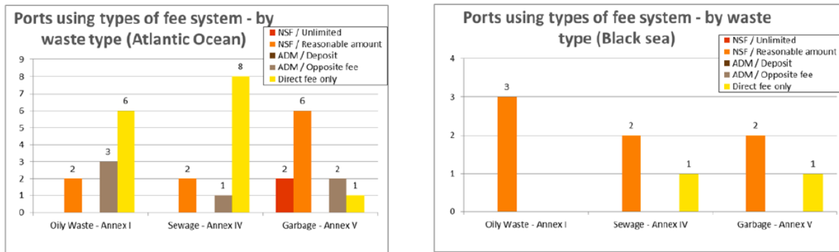
Figure 1: application of cost recovery systems in EU ports (source: Panteia/PwC)
