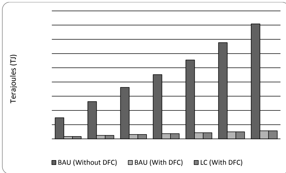
Figure 4-1: Future End-Use Energy Demand (TJ)
