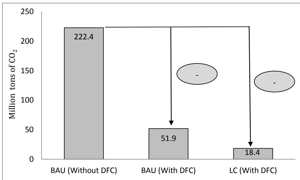
Figure 4-3: Reduction in Cumulative CO 2 emissions (2016-2046)
