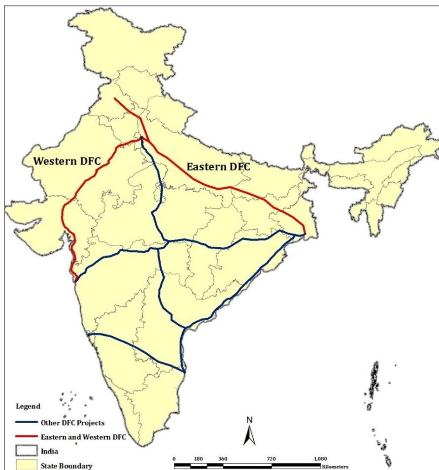
Figure 2-3: Proposed DFCs in India
