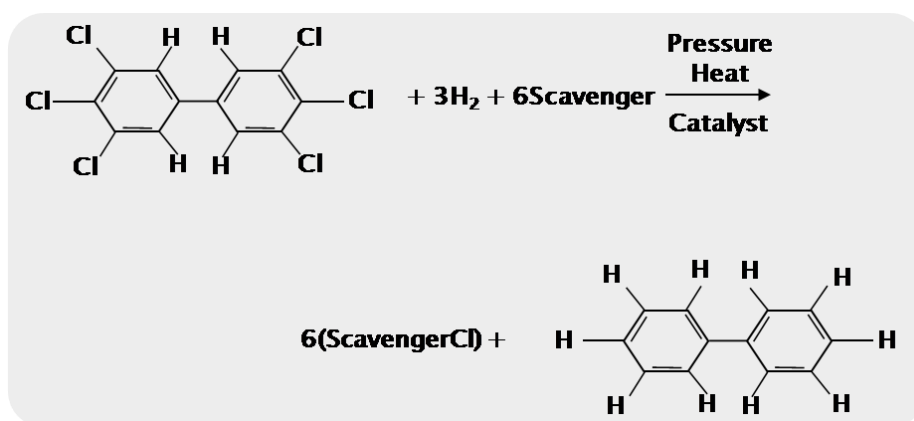
Figure 4. PCB reaction
