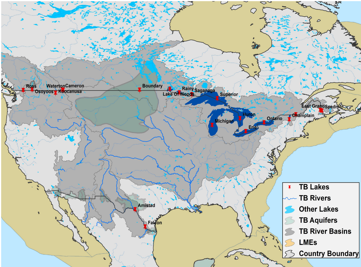
Figure 3.6 Transboundary Lakes in North America Region
