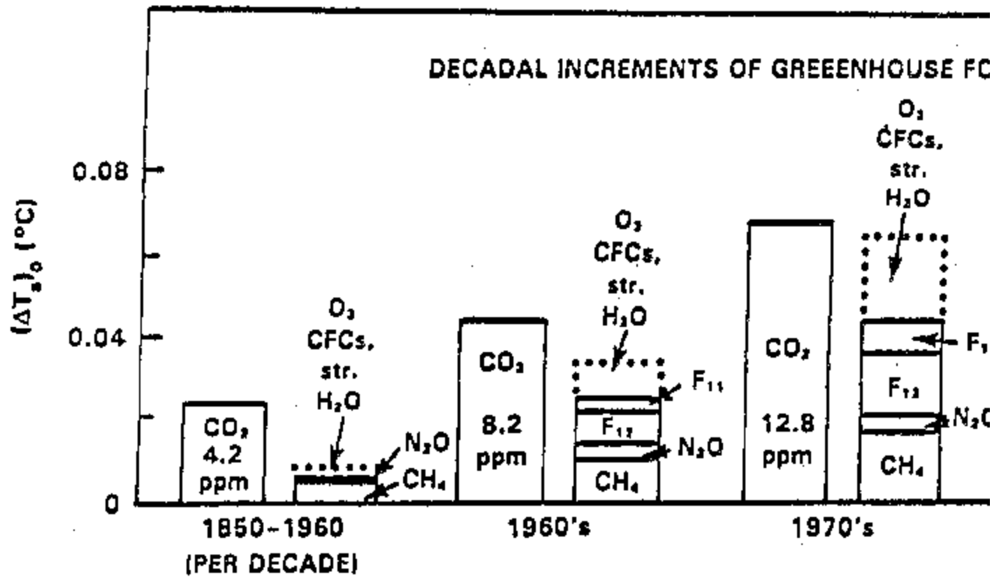
Figure 2. Decadal additions to global mean greenhouse forcing of the the computed temperature change at equilibrium ( t \rightarrow \infty ) for the estimated gas abundances, with no climate feedbacks included. (WMO, 1985).
