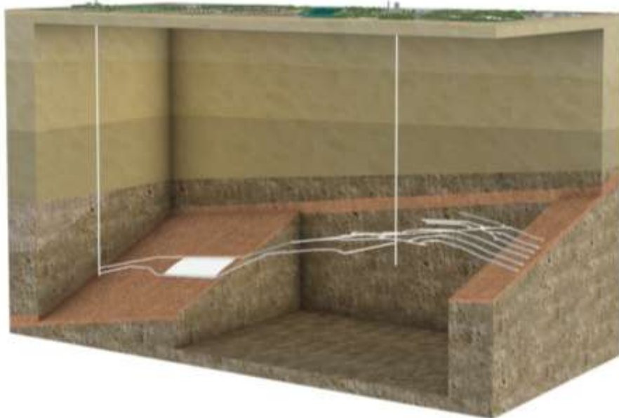
Figure 49 Model of the Konrad site showing the repository horizons and the overburden layers (source: Bundesamt für Strahlenschutz BfS [16]).
