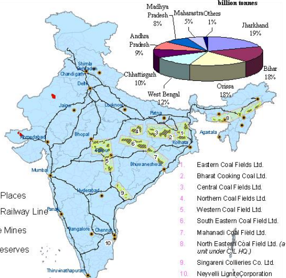
State Wise Coal Reserves Total Proven Reserves 959 billion tonnes
